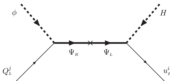
Figure 6: Top mass from an extended Higgs sector.
