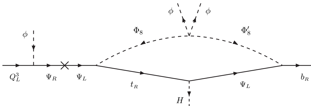
Figure 8: b -quark mass generated at one loop. The gauge-singlet scalar has a VEV \langle \phi \rangle \sim M_\Psi .
