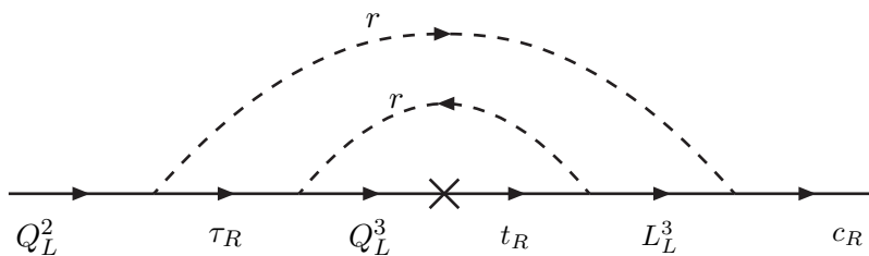
Figure 3: Charm mass induced by the 2-loop “rainbow” diagram involving the r scalar.
