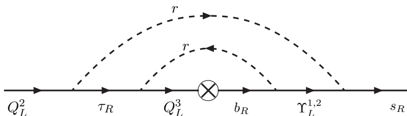
Figure 11: Strange mass induced by a 3-loop “rainbow” diagram. The \otimes symbol represents the b mass induced at 1-loop as in figure 8.
