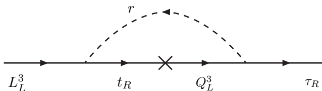
Figure 2: The 1-loop diagram responsible for the tau mass. The \times represents a top quark mass insertion.
