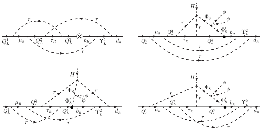
Figure 12: Down-quark mass induced at 4 loops. In the first diagram, the \otimes represents the 1-loop b -mass insertion of figure 8, and the upper two r lines do not intersect. The last two diagrams are also nonplanar (the lower two r lines do not intersect). As before the \bullet indicates a vertex obtained by integrating out the \Psi fermion.
