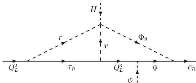
Figure 9: Charm-quark mass induced at 2 loops by the \Phi_8 interactions.
